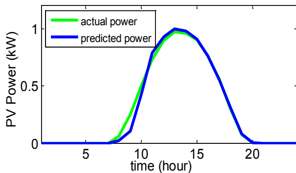
Figure 7: PV Generation Prediction
