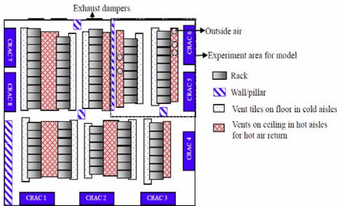
Figure 6: Data Center Layout
