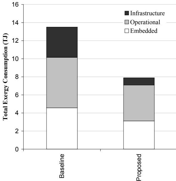
Figure 4: Overall exergy consumption across the lifecycle for a baseline and a lifecycle-based design.
